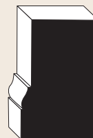
Brick Mould 1-1/4" x 2"
